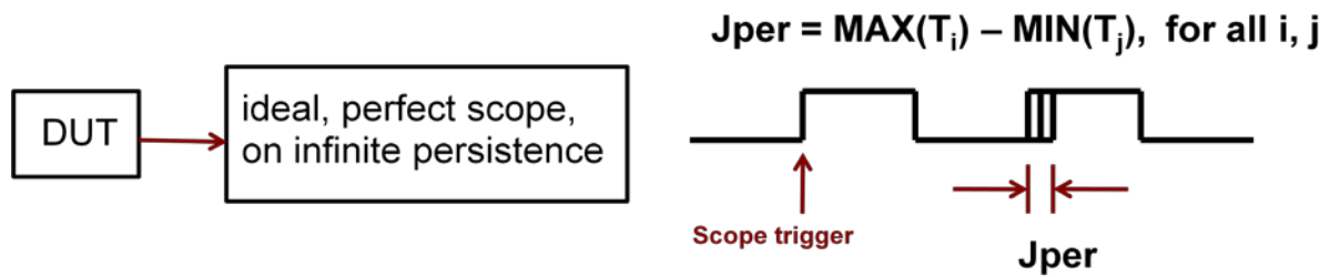
Figure 2: Period Jitter
