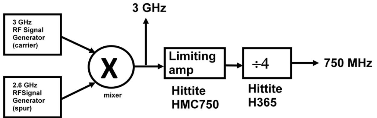
Figure 8: Aliasing Test Diagram
