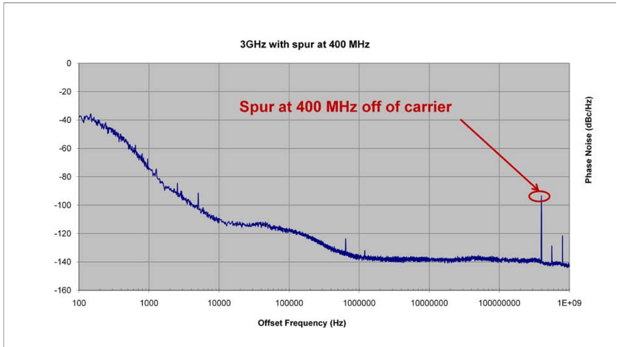
Figure 10: 3 GHz Phase Noise Plot
