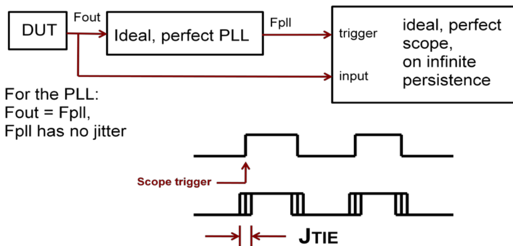
Figure 3: TIE Jitter
