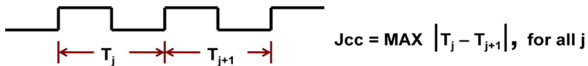
Figure 1: Cycle-to-Cycle Jitter
