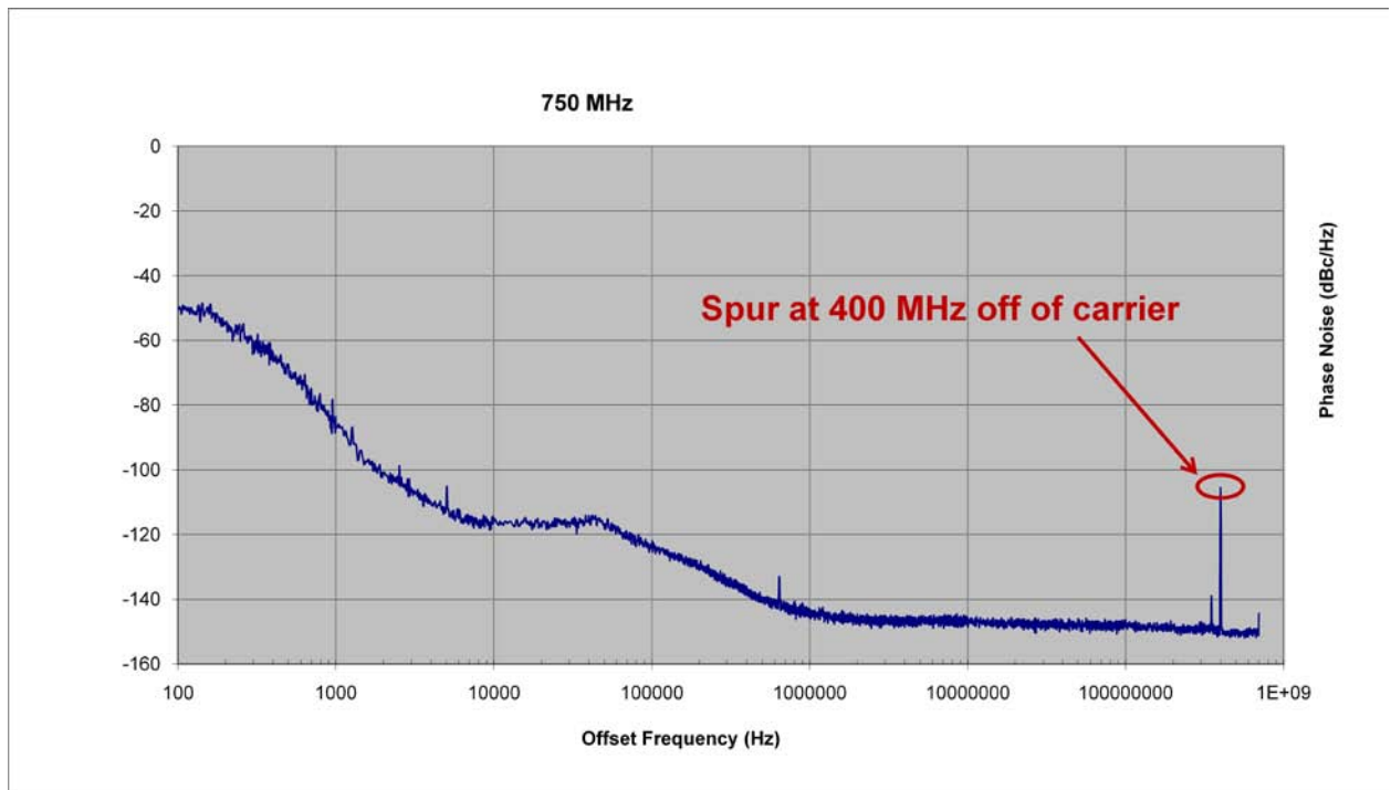
Figure 12: 750 MHz Phase Noise Plot
