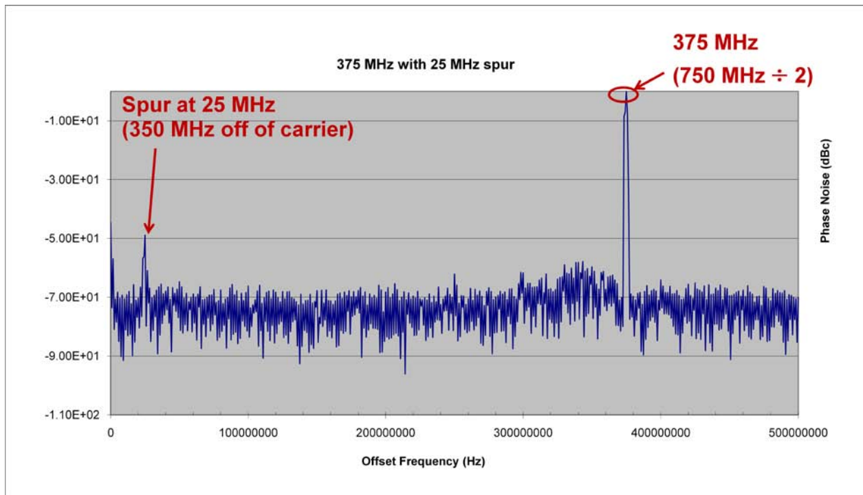
Figure 13: 375 MHz Spectrum
