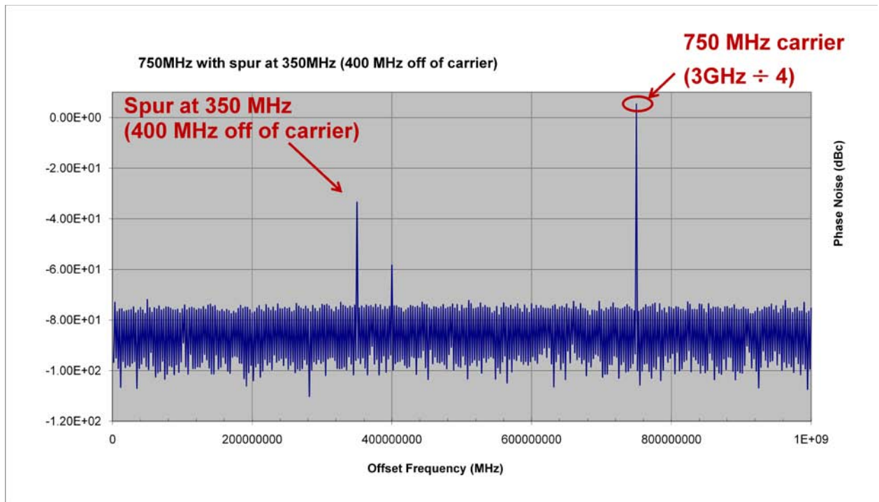
Figure 11: 750 MHz Spectrum
