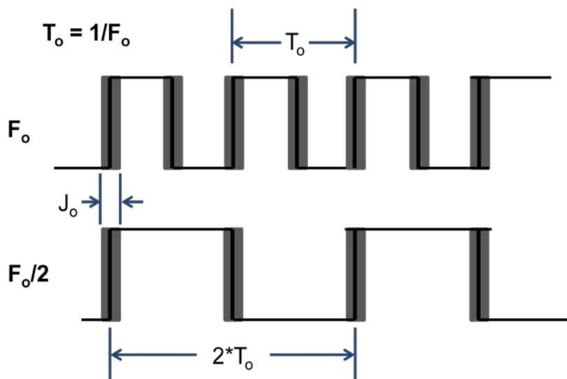
Figure 4: Division by Two
