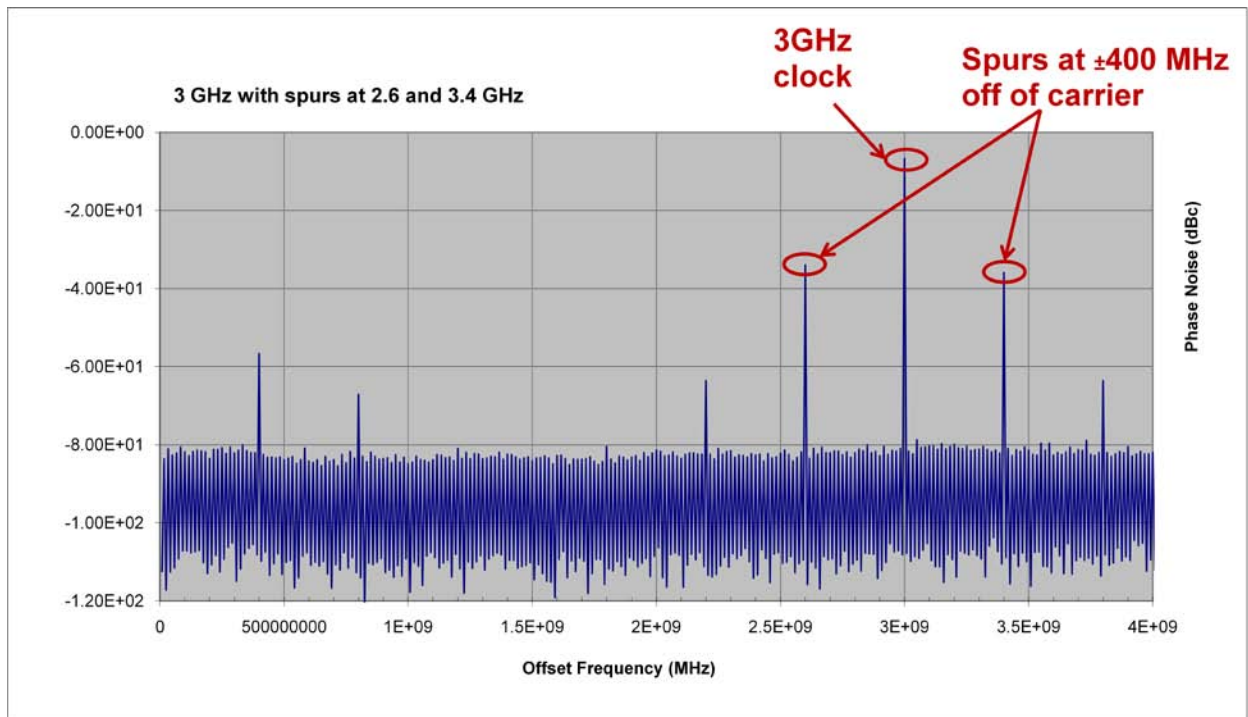
Figure 9: 3 GHz Spectrum
