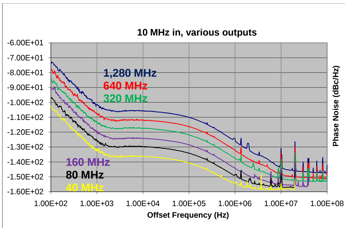
Figure 6: Phase Noise Plots for Different Divisor Values
